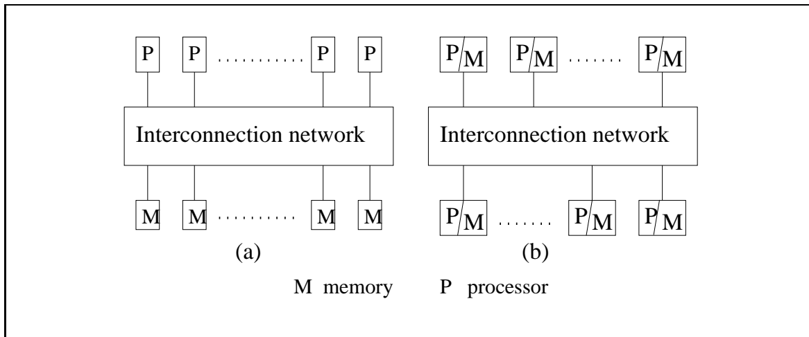
Figure 1.3: Two standard architectures for parallel systems. (a) Uniform memory access (UMA) multiprocessor system. (b) Non-uniform memory access (NUMA) multiprocessor. In both architectures, the processors may locally cache data from memory.
