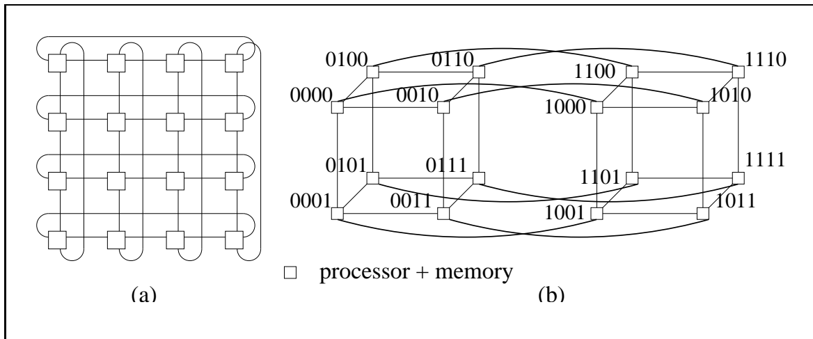
Figure 1.5: Some popular topologies for multicomputer shared-memory machines. (a) Wrap-around 2D-mesh, also known as torus. (b) Hypercube of dimension 4.
