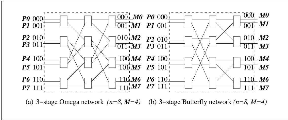
Figure 1.4: Interconnection networks for shared memory multiprocessor systems. (a) Omega network for n = 8 processors P0 - P7 and memory banks M0 - M7 . (b) Butterfly network for n = 8 processors P0 - P7 and memory banks M0 - M7 .
