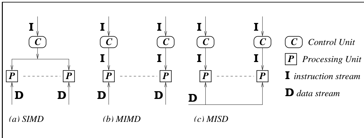
Figure 1.6: Flynn's taxonomy of SIMD, MIMD, and MISD architectures for multiprocessor/multicomputer systems.
