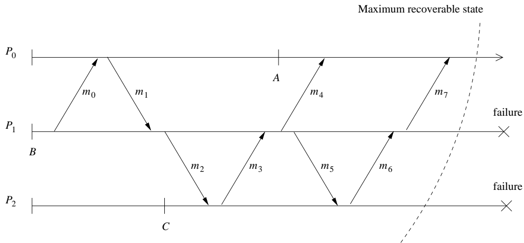
Figure 13.8: Pessimistic logging.
