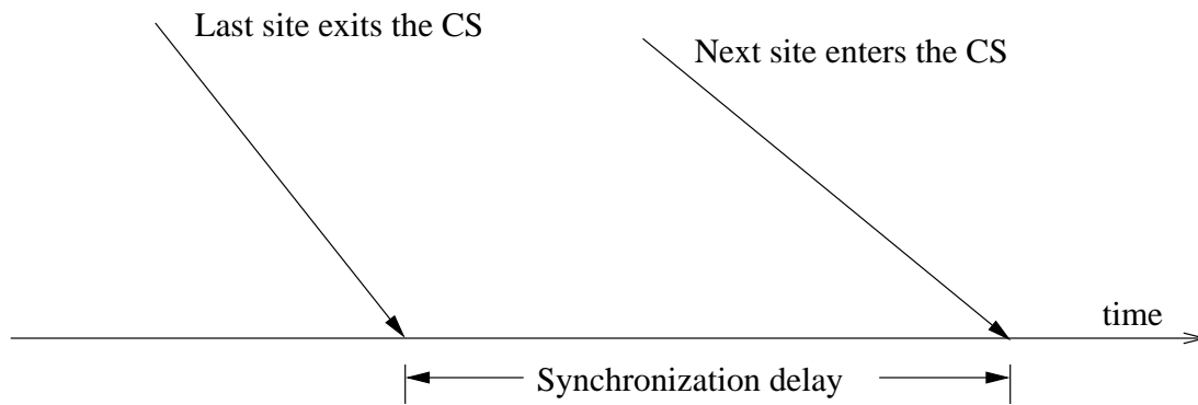
Figure 9.1: Synchronization Delay
