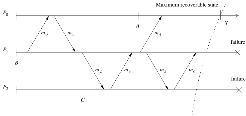
Figure 13.10: Causal logging
