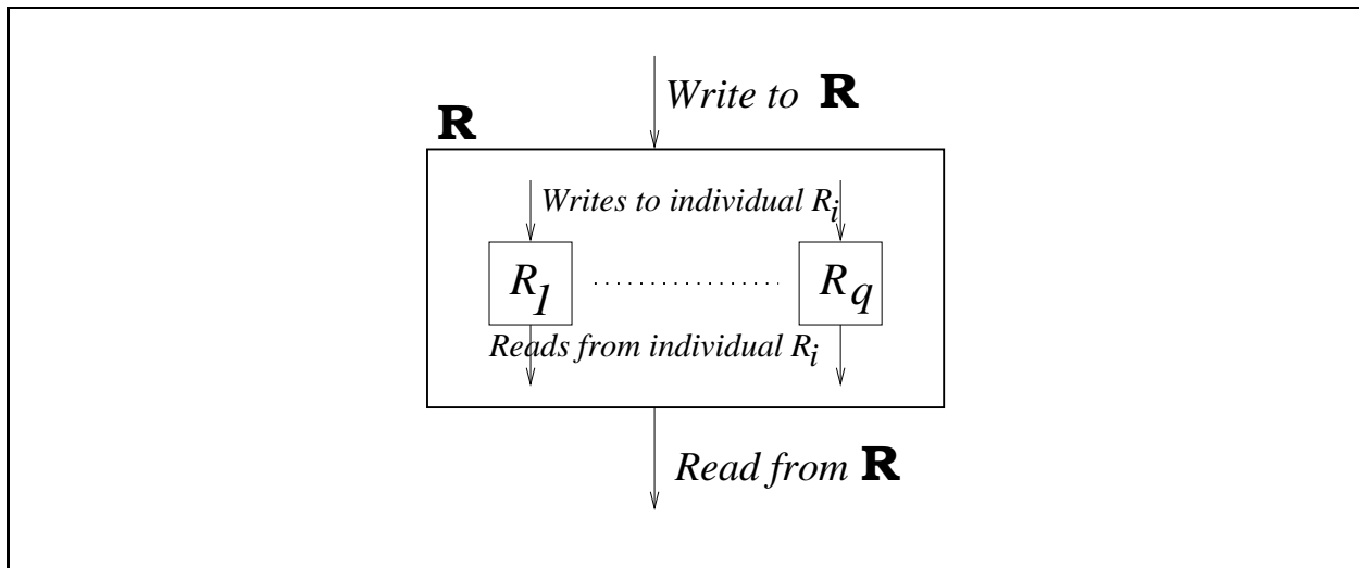
Figure 12.20: Register simulations.
