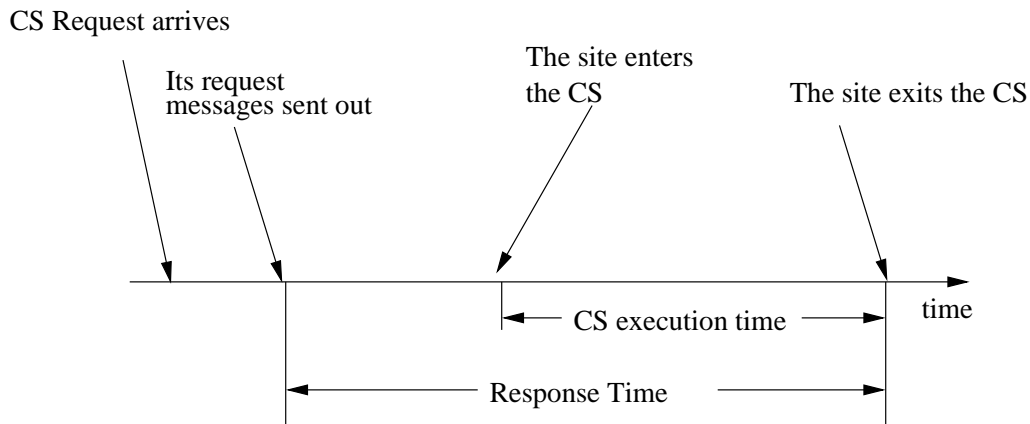
Figure 9.2: Response Time
