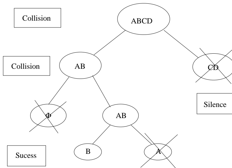
Figure 17.5: An example.
