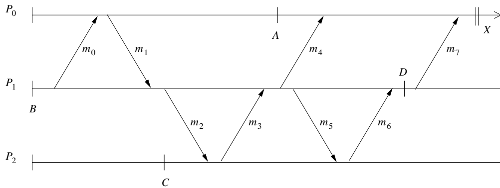
Figure 13.9: Optimistic logging.
