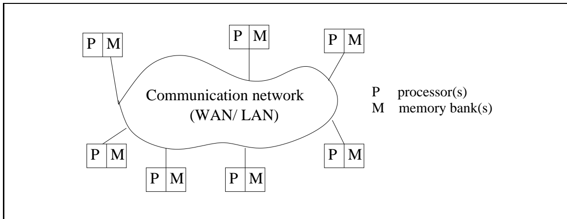
Figure 1.1: A distributed system that connects processors by a communication network.
